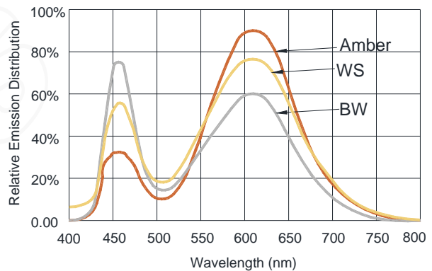
Wavelength Characteristics
