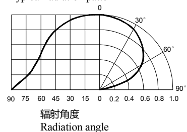
典型的辐射方向图 120° Typical radiation pattern 120°
