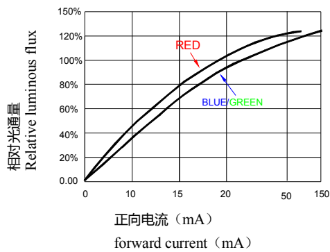
相对光通量与正向电流的关系 The relationship between relative luminous flux and forward current
